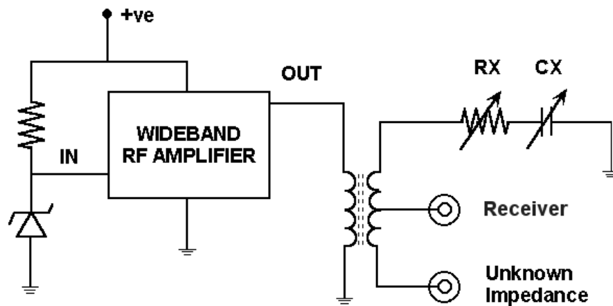
Figure 12 – Noise Bridge.
